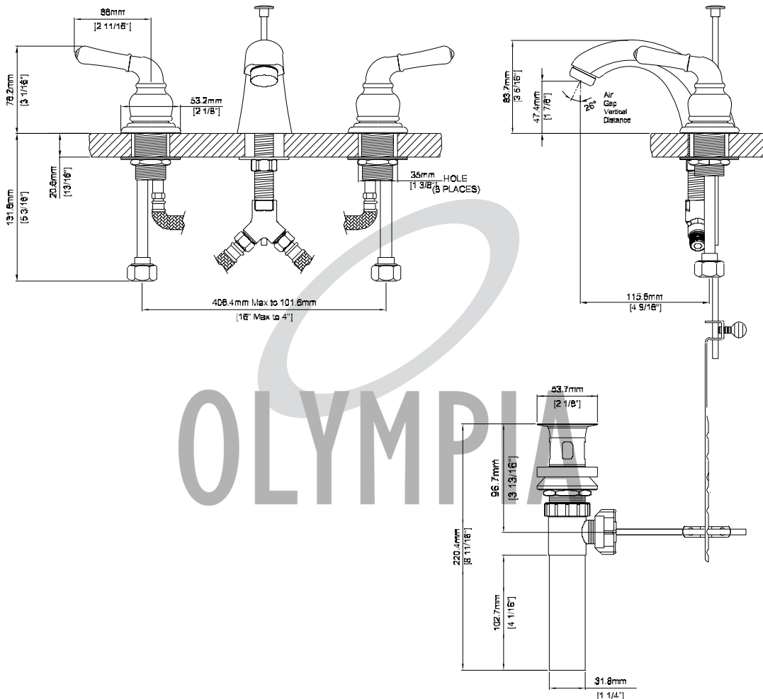
50/50 Pop-Up Drain
